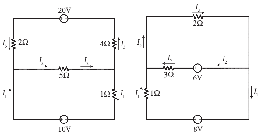
Figure 1.5 Circuits for use in exercises 35 and 36.
