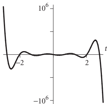
Figure 8.2 The degree 11 Hermite polynomial, H_{11}(t) , plotted on the interval [-3, 3] .
