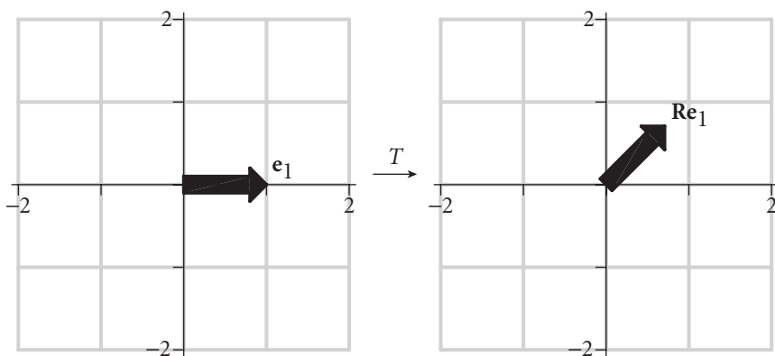
Figure 1.17 The vectors \mathbf{e}_1 and T(\mathbf{e}_1) = \mathbf{R}\mathbf{e}_1 .
