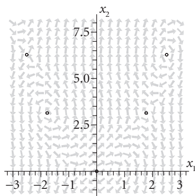
Figure 6.10 The direction field for the system (6.3.16) with equilibrium points (0, 0) , (-\sqrt{\pi}, \pi) , (\sqrt{\pi}, \pi) , (-\sqrt{2\pi}, 2\pi) , and (\sqrt{2\pi}, 2\pi) .
