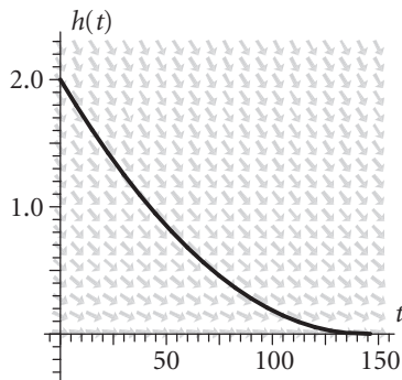
Figure 2.12 The slope field for dh/dt = -0.019676\sqrt{h} .
