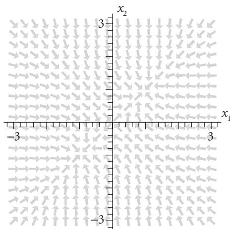
Figure 6.3 The direction field for the system \mathbf{x}' = \mathbf{F}(\mathbf{x}) given in (6.2.1).
