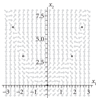
Figure 6.6 The direction field for the system (6.2.7) with equilibrium points (0, 0) , (-\sqrt{\pi}, \pi) , (\sqrt{\pi}, \pi) , (-\sqrt{2\pi}, 2\pi) , and (\sqrt{2\pi}, 2\pi) .
