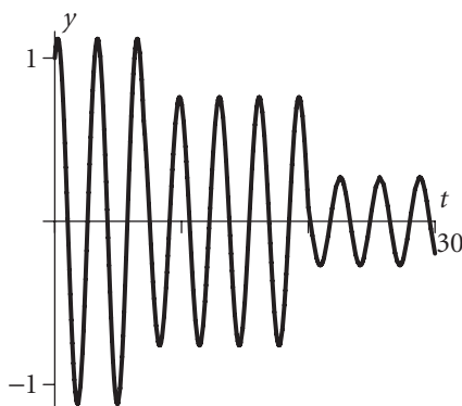
Figure 5.11 The solution to the IVP of example 5.5.5.
