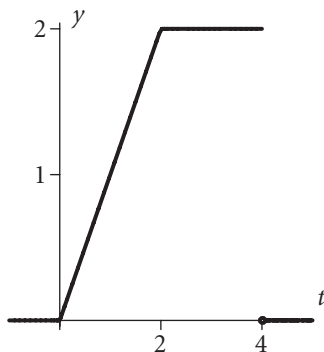
Figure 5.4 The function f(t) in example 5.4.1.
