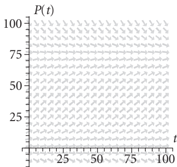
Figure 2.10 The slope field for dP/dt = 0.05P(1 - P/75) .
