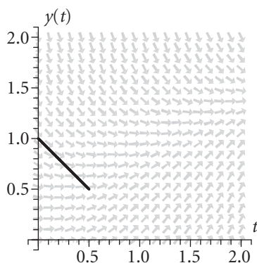
Figure 2.6 Taking one step to estimate y(0.5) in (2.6.1).
