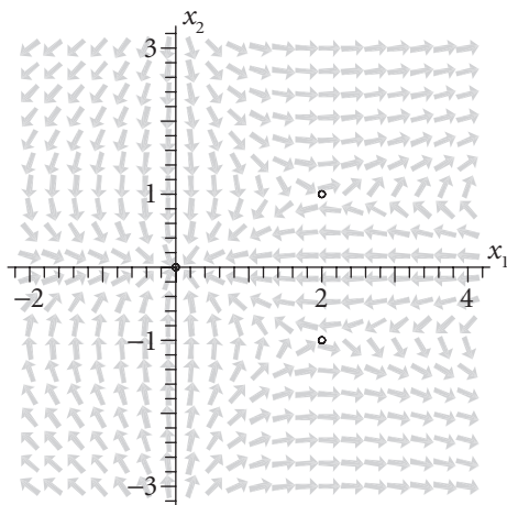
Figure 6.7 The direction field for the system (6.2.10) with equilibrium points (0, 0) , (2, 1) , and (2, -1) .
