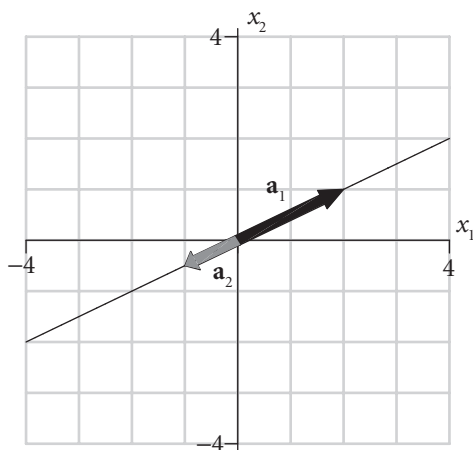
Figure 1.11 Linear combinations of \mathbf{a}_1 and \mathbf{a}_2 from example 1.6.1.
