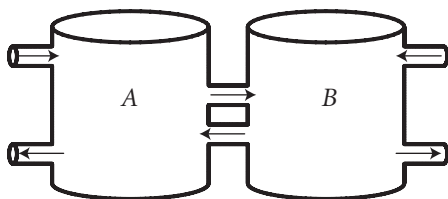
Figure 1.1 Two tanks with inflows, outflows, and connecting pipes.
