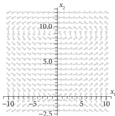
Figure 6.9 The direction field for Example 6.3.2.
