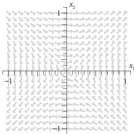
Figure 6.5 The direction field for the linear system \mathbf{x}' = \mathbf{A}\mathbf{x} given in (6.2.5).
