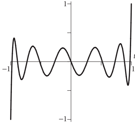
Figure 8.1 The degree 11 Legendre polynomial, P_{11}(t) .
