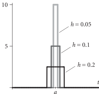
Figure 5.5 The forcing function F_h(t) for h = 0.2 , h = 0.1 , and h = 0.05 .
