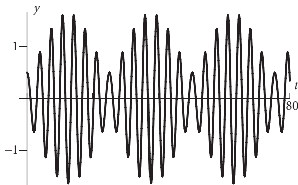
Figure 4.4 The solution to the IVP in example 4.5.2.
