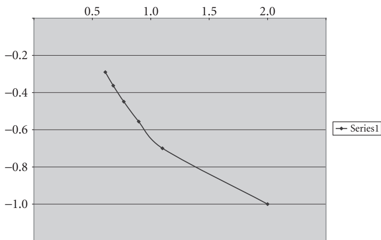
Figure 6.12 An Excel plot of an approximate solution to the IVP (6.4.14).
