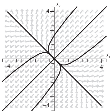
Figure 3.6 The direction field for the system \mathbf{x}' = \mathbf{Ax} of example 3.4.1 along with several trajectories.
