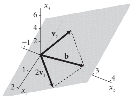
Figure 1.7 The parallelogram formed by the vectors 2\mathbf{v}_1 and \mathbf{v}_2 from (1.3.6).
