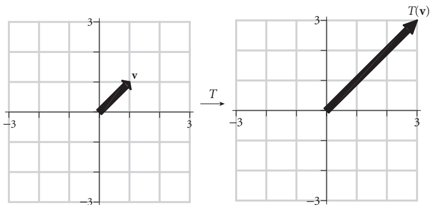
Figure 1.16 The vectors \mathbf{v} and T(\mathbf{v}) .
