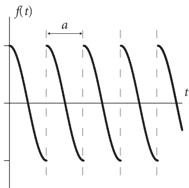
Figure 5.13 A periodic function with period a that is piecewise continuous.
