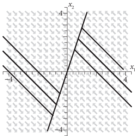
Figure 3.9 The direction field for the system \mathbf{x}' = \mathbf{A}\mathbf{x} of example 3.4.4 along with several trajectories.
