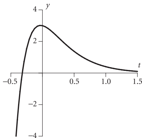
Figure 4.1 A plot of the solution y(t) to the IVP given in (4.2.11).
