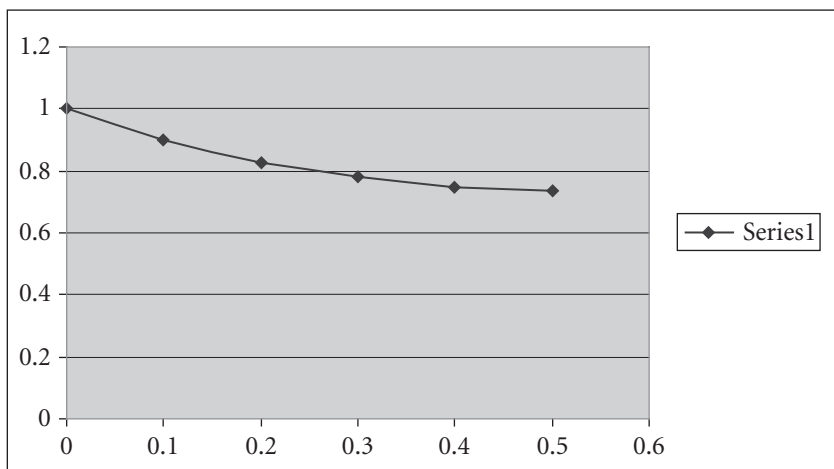
Figure 2.9 An Excel plot of an approximate solution to the IVP y' = t - y^2 , y(0) = 1 , for 0 \leq t \leq 0.5 .
