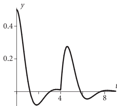
Figure 5.2 The solution curve y(t) to (5.1.3).
