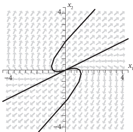
Figure 3.11 The direction field for the system \mathbf{x}' = \mathbf{A}\mathbf{x} of example 3.5.2 along with several trajectories.
