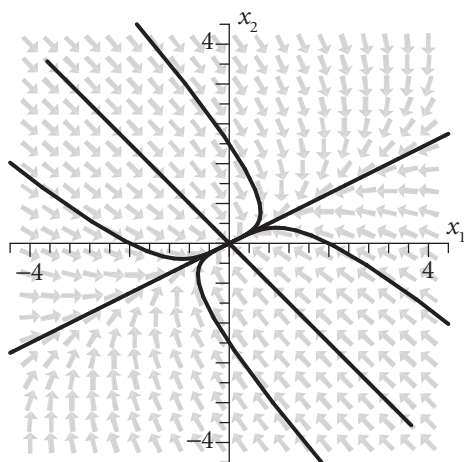
Figure 3.7 The direction field for the system \mathbf{x}' = \mathbf{A}\mathbf{x} in example 3.4.2 along with several trajectories.
