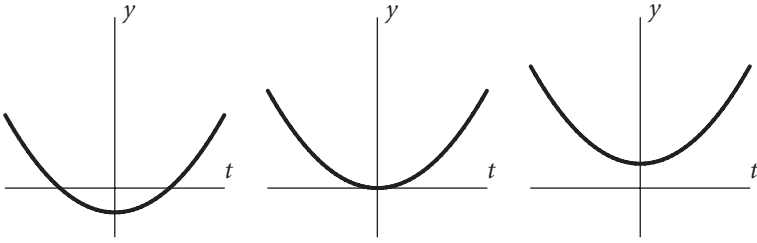
Figure C.1 Three concave up quadratic functions whose vertices lie, respectively, below, on, and above the t -axis.
