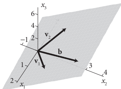
Figure 1.6 The vectors \mathbf{v}_1, \mathbf{v}_2 , and \mathbf{b} from (1.3.6).
