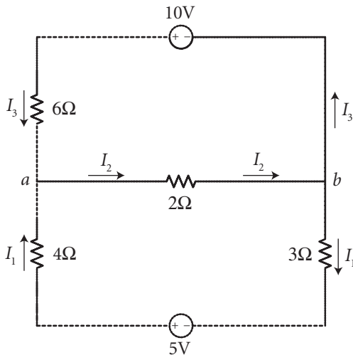
Figure 1.2 A simple circuit with two loops, two batteries, and four resistors.
