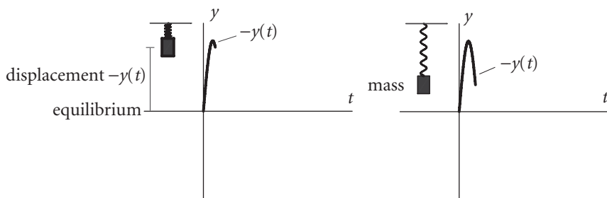
Figure 3.2 A spring-mass system shown at two different points in time; -y(t) denotes the displacement of the mass from equilibrium (where displacements below the t -axis are considered positive).
