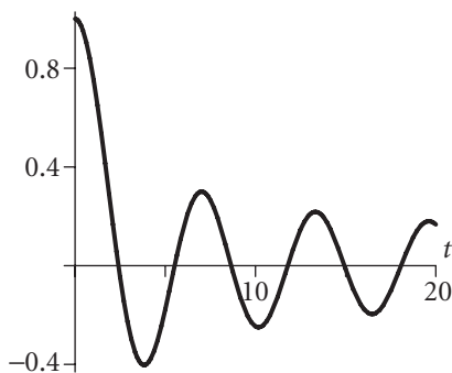
Figure 8.4 The Bessel function of the first kind, J_0(t) .
