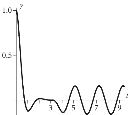
Figure 5.10 The solution to the IVP in example 5.5.4.
