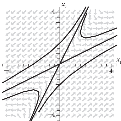
Figure 3.8 The direction field for the system \mathbf{x}' = \mathbf{A}\mathbf{x} of example 3.4.3 along with several trajectories.
