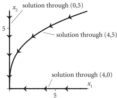
Figure 3.3 Plots of solutions to three IVPs for the system in example 3.2.1. Arrows indicate the direction of flow along the solution curve as time increases.
