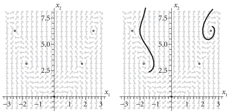
Figure 6.8 At left, the direction field for the system (6.2.7) with equilibrium points (0, 0) , (-\sqrt{\pi}, \pi) , (\sqrt{\pi}, \pi) , (-\sqrt{2\pi}, 2\pi) , and (\sqrt{2\pi}, 2\pi) . At the right, the same direction field with trajectories through (2, 6) and (-2, 6) is included.
