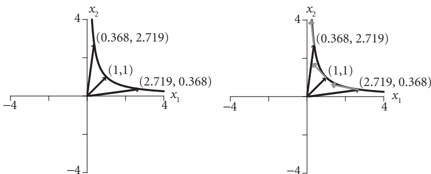
Figure 3.4 At left, the solution curve \mathbf{x}(t) given in (3.4.1). At right, the solution curve \mathbf{x}(t) given in (3.4.1), along with corresponding scaled derivative vectors at times t = -1 , t = 0 , and t = 1 .
