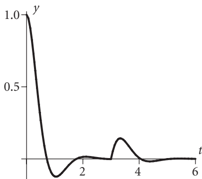
Figure 5.6 The solution to the IVP (5.4.14).
