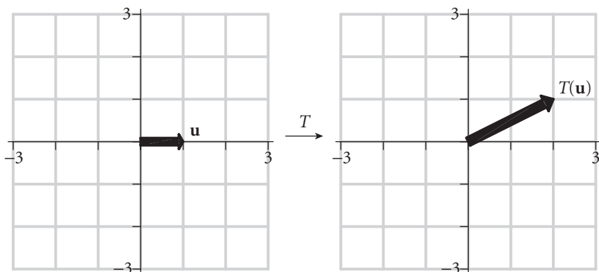
Figure 1.15 The vectors \mathbf{u} and T(\mathbf{u}) in example 1.10.1.
