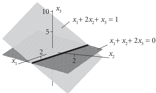
Figure 1.3 The intersection of the planes x_1 + 2x_2 + x_3 = 1 and x_1 + x_2 + 2x_3 = 0 .
