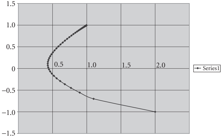
Figure 6.11 The trajectory for the IVP (6.4.11) generated by Euler's method with h = 0.1 .
