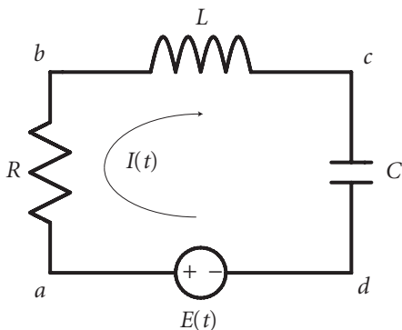
Figure 3.17 An RLC circuit with resistance R , inductance L , capacitance C , and energy source E(t) .
