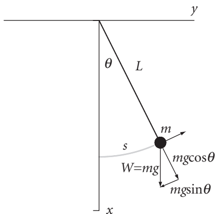
Figure 6.2 Component of gravity's force along the pendulum's motion.
