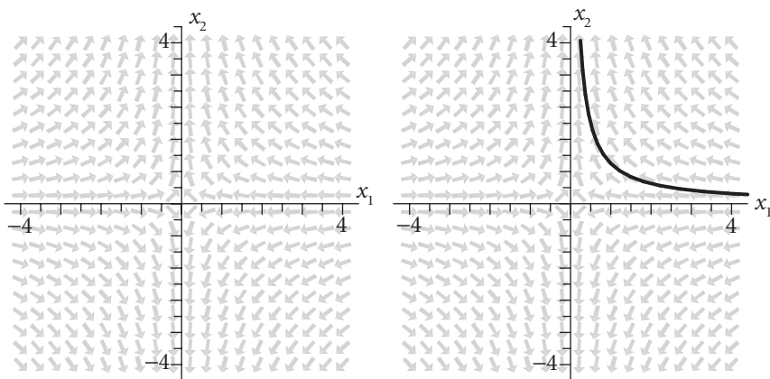
Figure 3.5 At left, the direction field for the system \mathbf{x}' = \mathbf{A}\mathbf{x} given by (3.4.5). At right, the solution to (3.4.5) that is given by (3.4.1).
