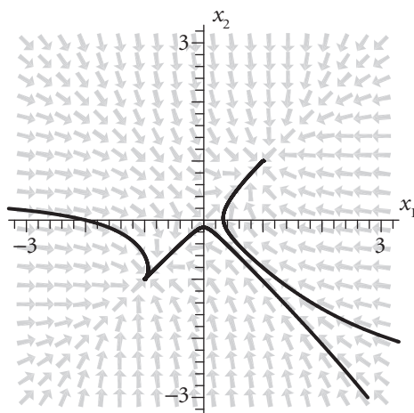
Figure 6.4 The direction field for the system \mathbf{x}' = \mathbf{F}(\mathbf{x}) given in (6.2.1) with three trajectories.
