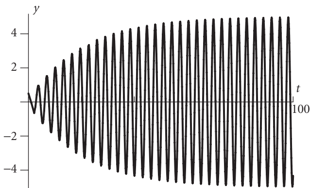
Figure 4.6 The solution to the IVP in example 4.5.4.
