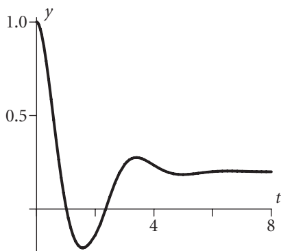
Figure 5.9 The solution y(t) to the IVP in example 5.5.3.
