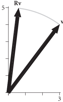
Figure 1.13 The vectors \mathbf{v} = [3 \ 4] and \mathbf{Rv} = [0.598 \ 4.964]^T .
