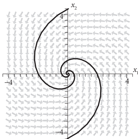
Figure 3.13 The direction field for the system \mathbf{x}' = \mathbf{A}\mathbf{x} of example 3.5.4 along with several trajectories.
