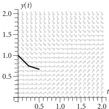
Figure 2.7 Two steps of size 0.25 to estimate y(0.5) in (2.6.1).
