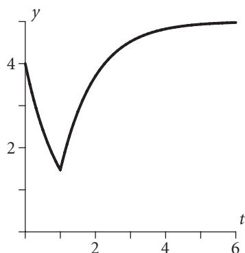
Figure 5.8 The solution to the IVP of example 5.5.2.
