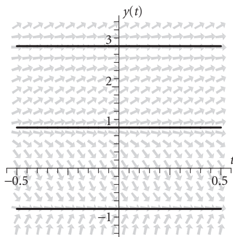
Figure 2.3 The slope field for y' = (y^2 - 1)(y - 3)^2 along with its three equilibrium solutions.
