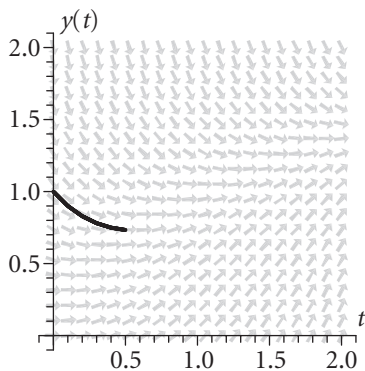
Figure 2.8 Five steps of size h = 0.1 to estimate y(0.5) .
