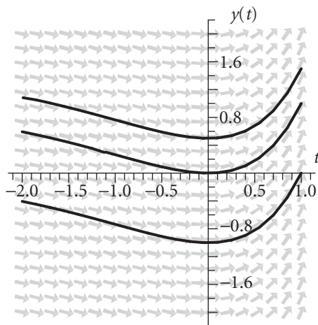
Figure 2.2 The slope field for (2.2.6) along with three solution functions for the initial conditions y(0) = 1/2 , y(0) = 0 , and y(0) = -1 .
