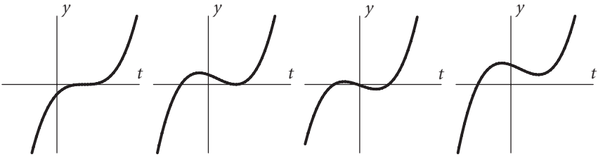
Figure C.2 Four cubic polynomials that demonstrate possible arrangements of the zeros of cubic functions.
