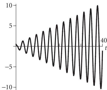
Figure 4.5 The solution to the IVP in example 4.5.3.
