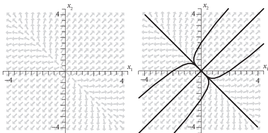
Figure 3.10 At left, the direction field for the system \mathbf{x}' = \mathbf{A}\mathbf{x} of example 3.4.1. At right, the same direction field with several trajectories.
