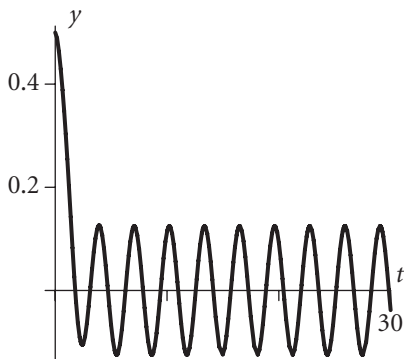
Figure 4.7 The solution to the IVP in example 4.5.5.
