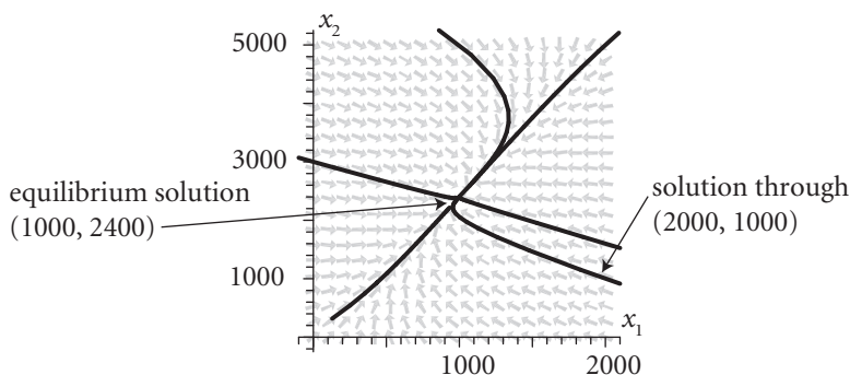
Figure 3.14 The direction field for the system \mathbf{x}' = \mathbf{A}\mathbf{x} + \mathbf{b} of example 3.6.1.
