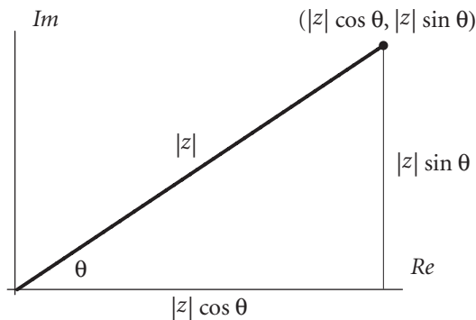
Figure B.2 The complex number z = |z|\cos\theta + i|z|\sin\theta .
