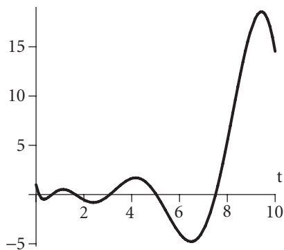
Figure 8.3 The degree 11 Laguerre polynomial L_{11}(t) plotted on the interval [0, 10] .
