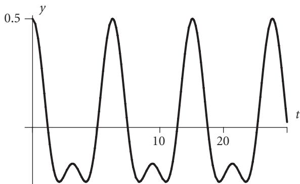
Figure 4.3 The solution y to the IVP in example 4.5.1.
